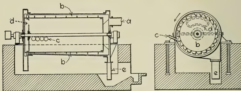
FIG. 67.—Thiesen Centrifugal Scrubber.
